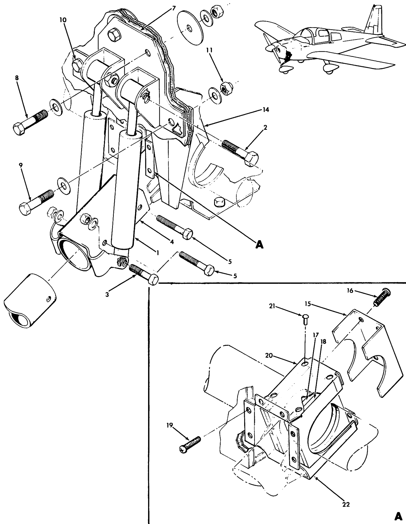
Shock Absorber Installation Figure 32-11
