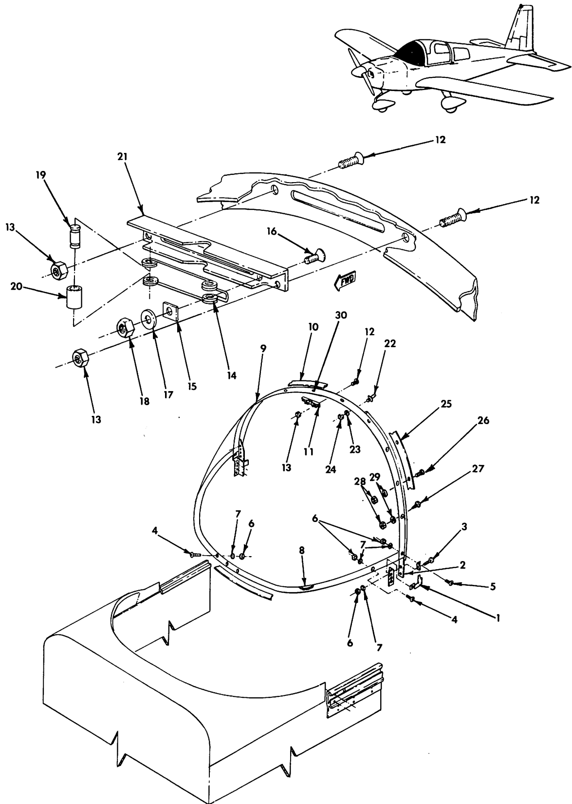
Windshield Installation Figure 56-1
