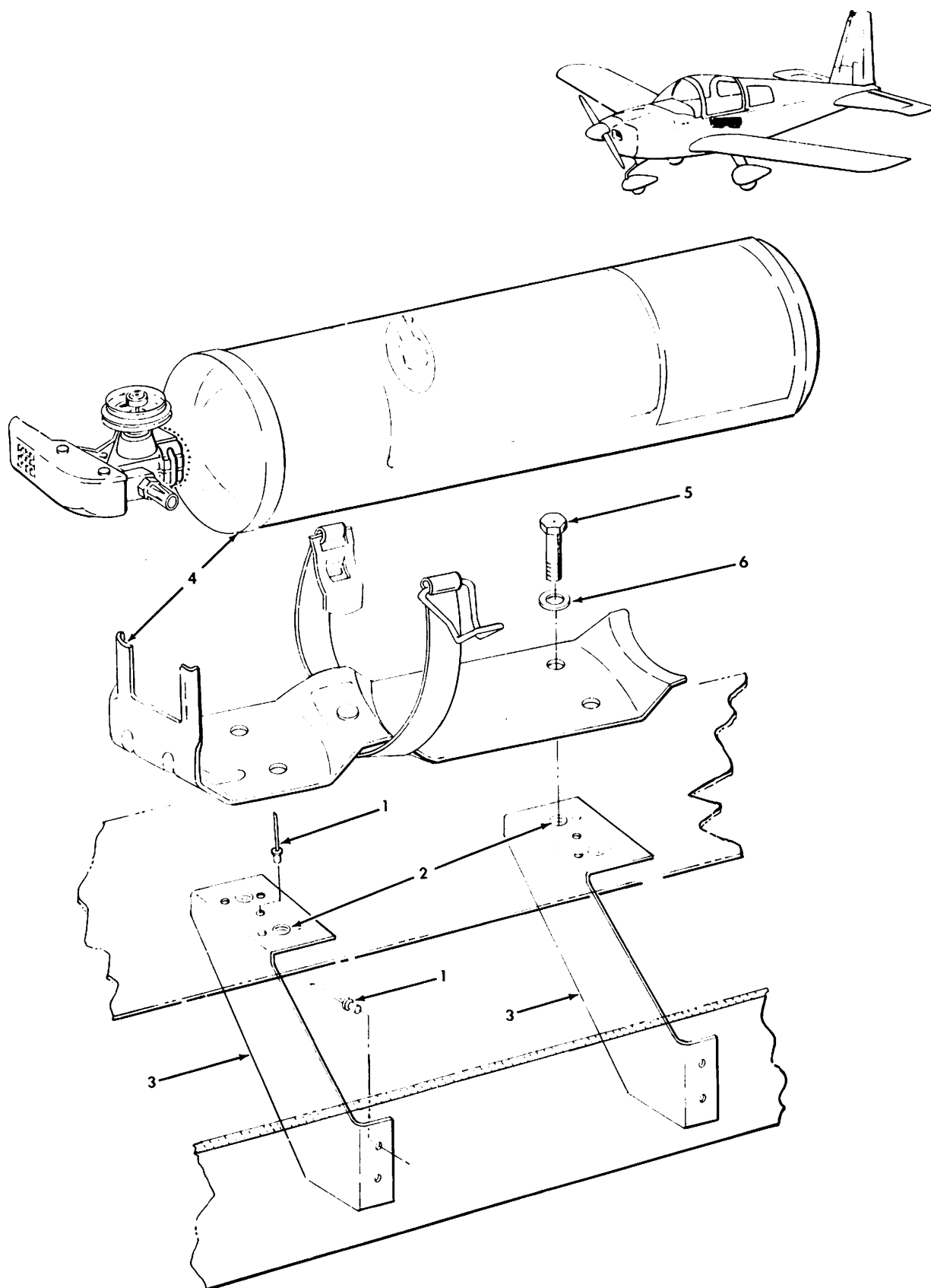
Fire Extinguisher Installation Figure 25-7
