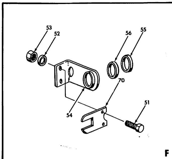
Wing Assembly and Installation (Sheet 2 of 2) Figure 57-1
