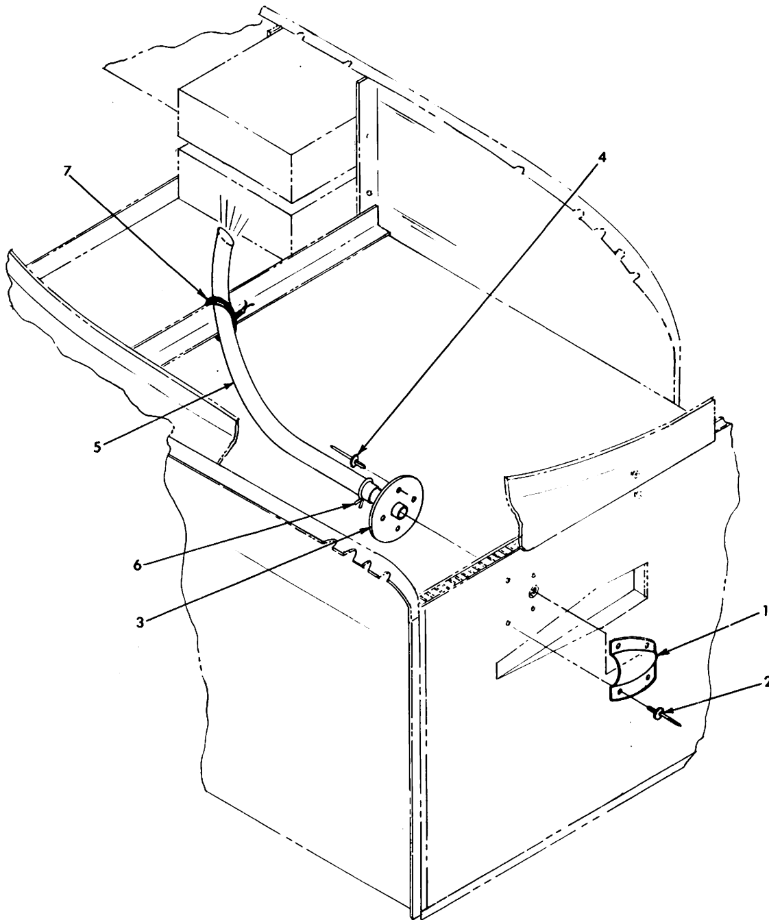
Radio Cooling Kit Installation Figure 21-3
