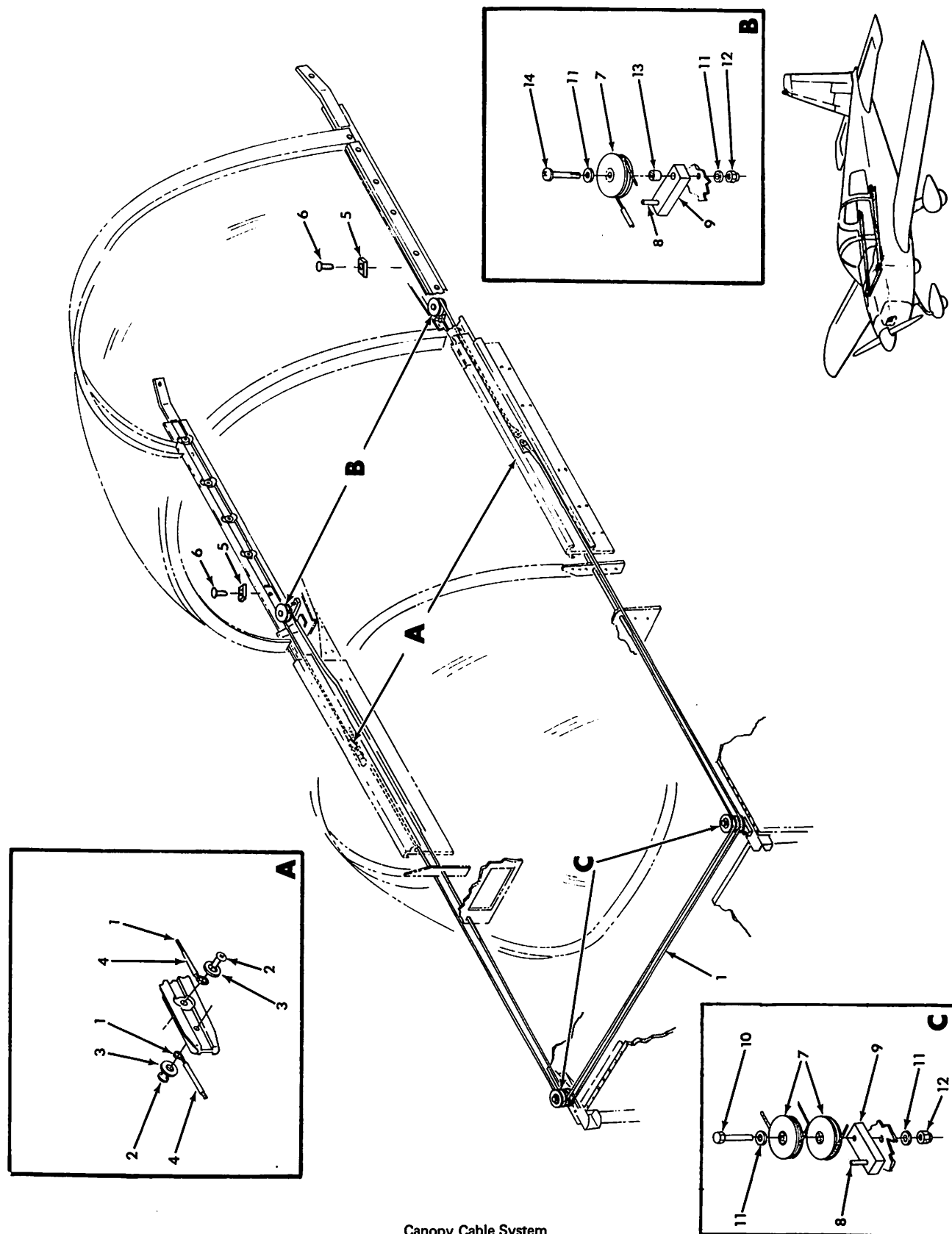
Canopy Cable System Figure 52-2
