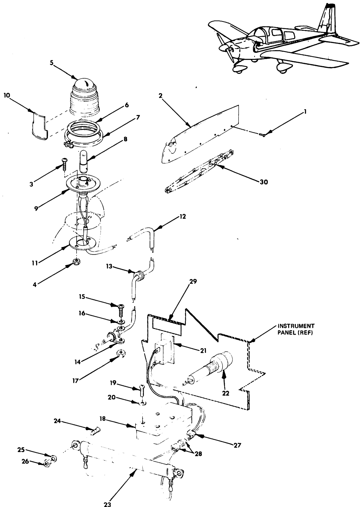
Flashing Beacon Installation Figure 33-4
