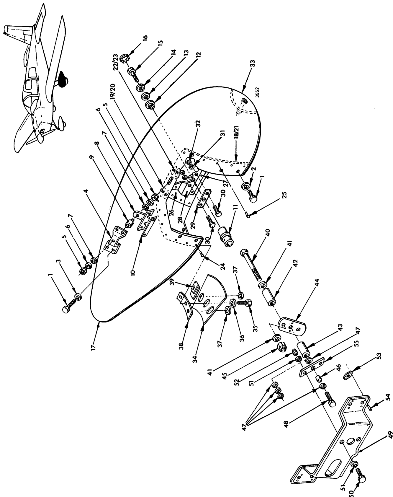
Main Wheel Fairing Figure 32-2
