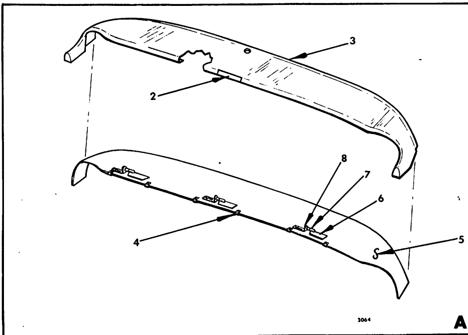
Instrument Panel Installation (Sheet 1 of 2) Figure 34-5
