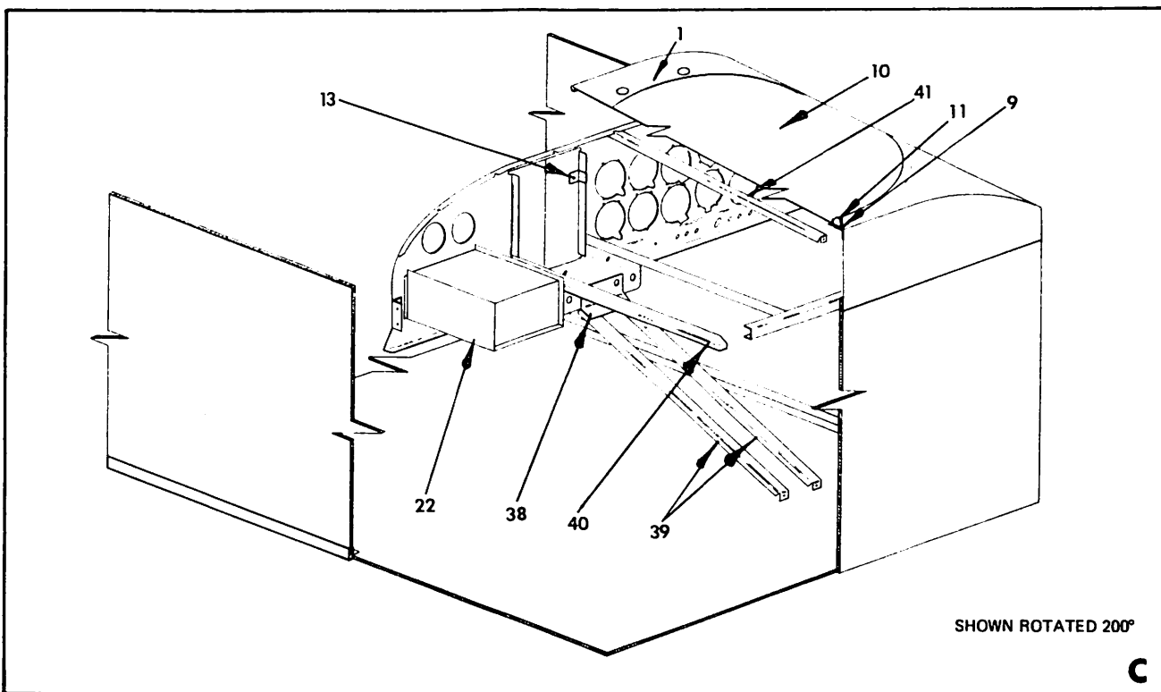
Instrument Panel Installation (Sheet 2 of 2) Figure 34-5
