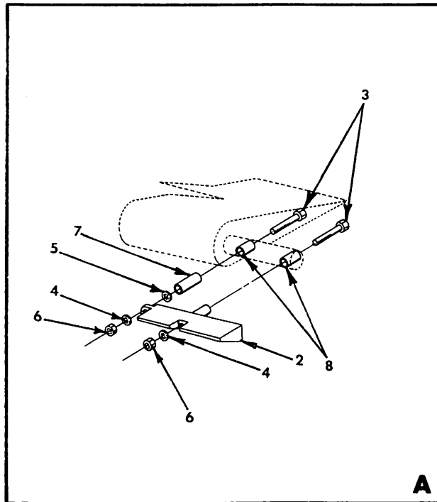
Aileron Assembly Figure 57-5
