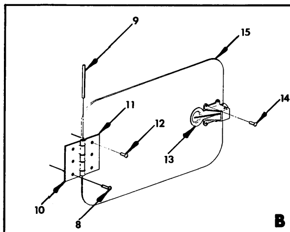
Upper Cowl Assembly Figure 71-2
