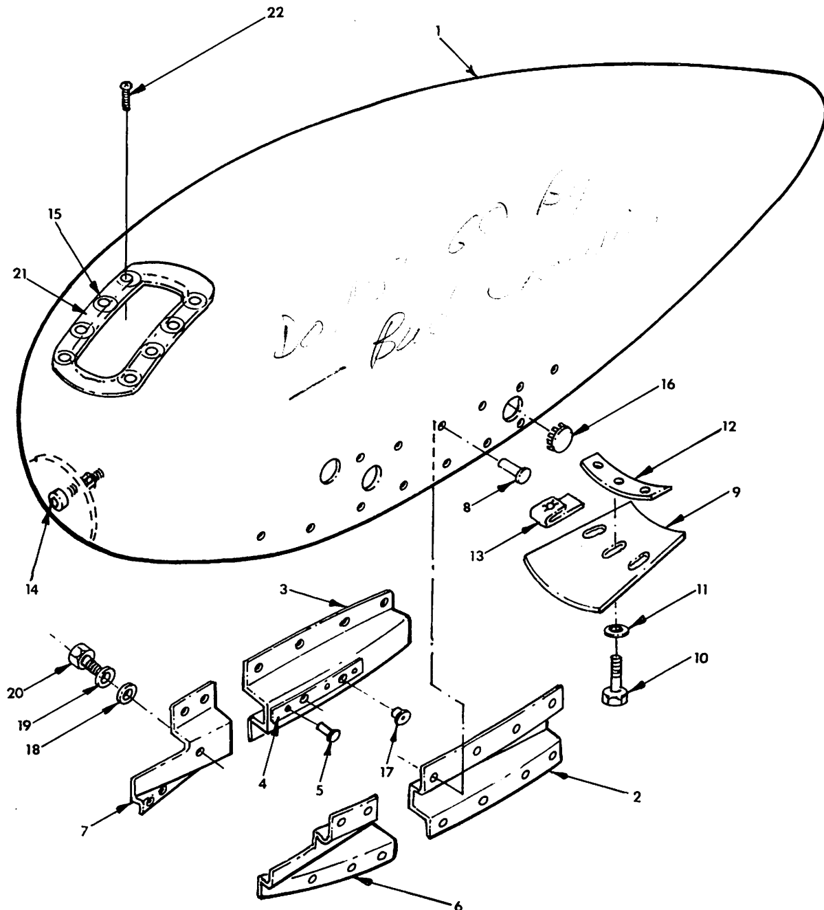
Nose Wheel Fairing Installation Figure 32-3
