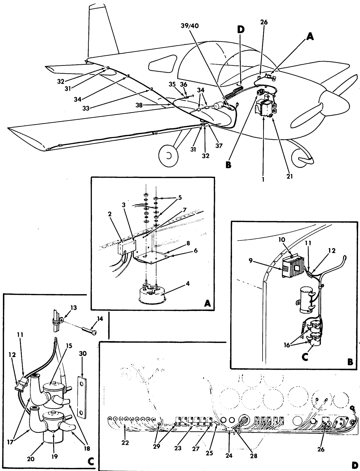
Electrical System Installation Figure 24-1
