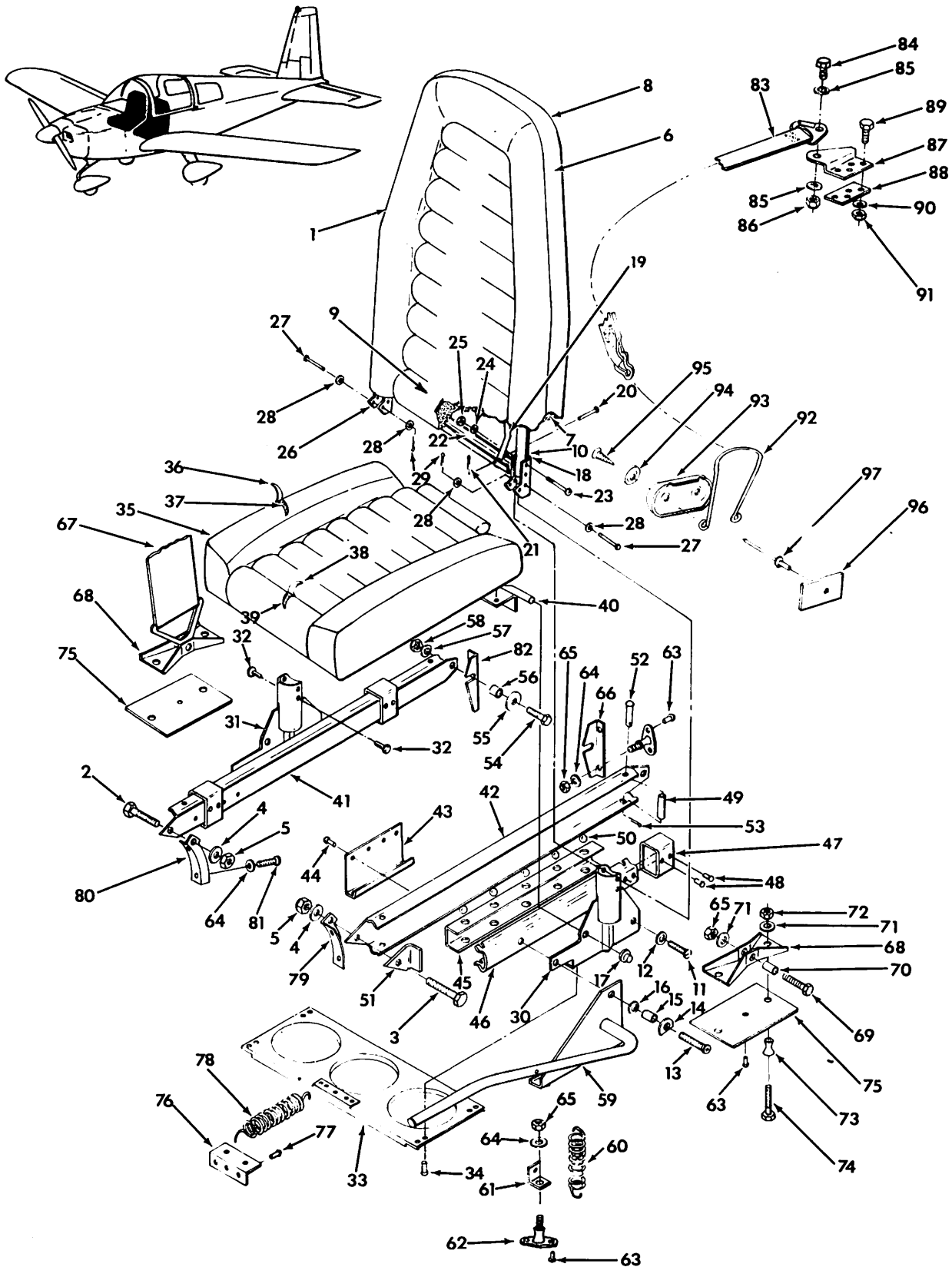
Seat and Harness Installation Figure 25-2
