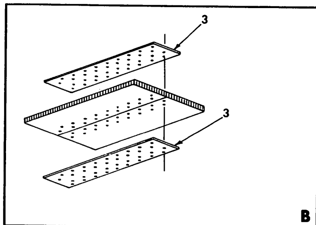
Lower Forward Fuselage Repair Section Figure 53-5
