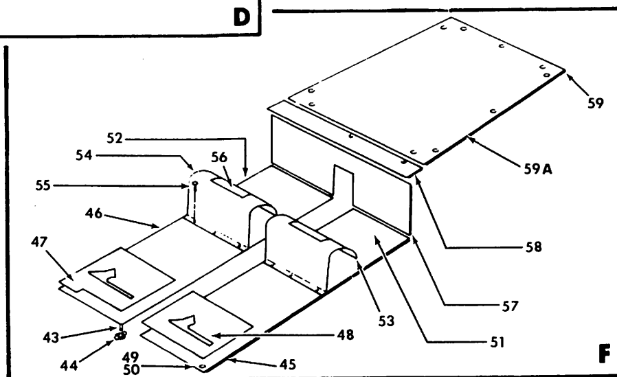
Upholstery and Insulation Installation (Sheet 2 of 2) Figure 25-4
