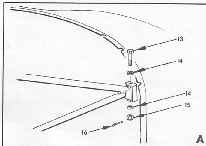
Power Plant Installation Figure 71-1
