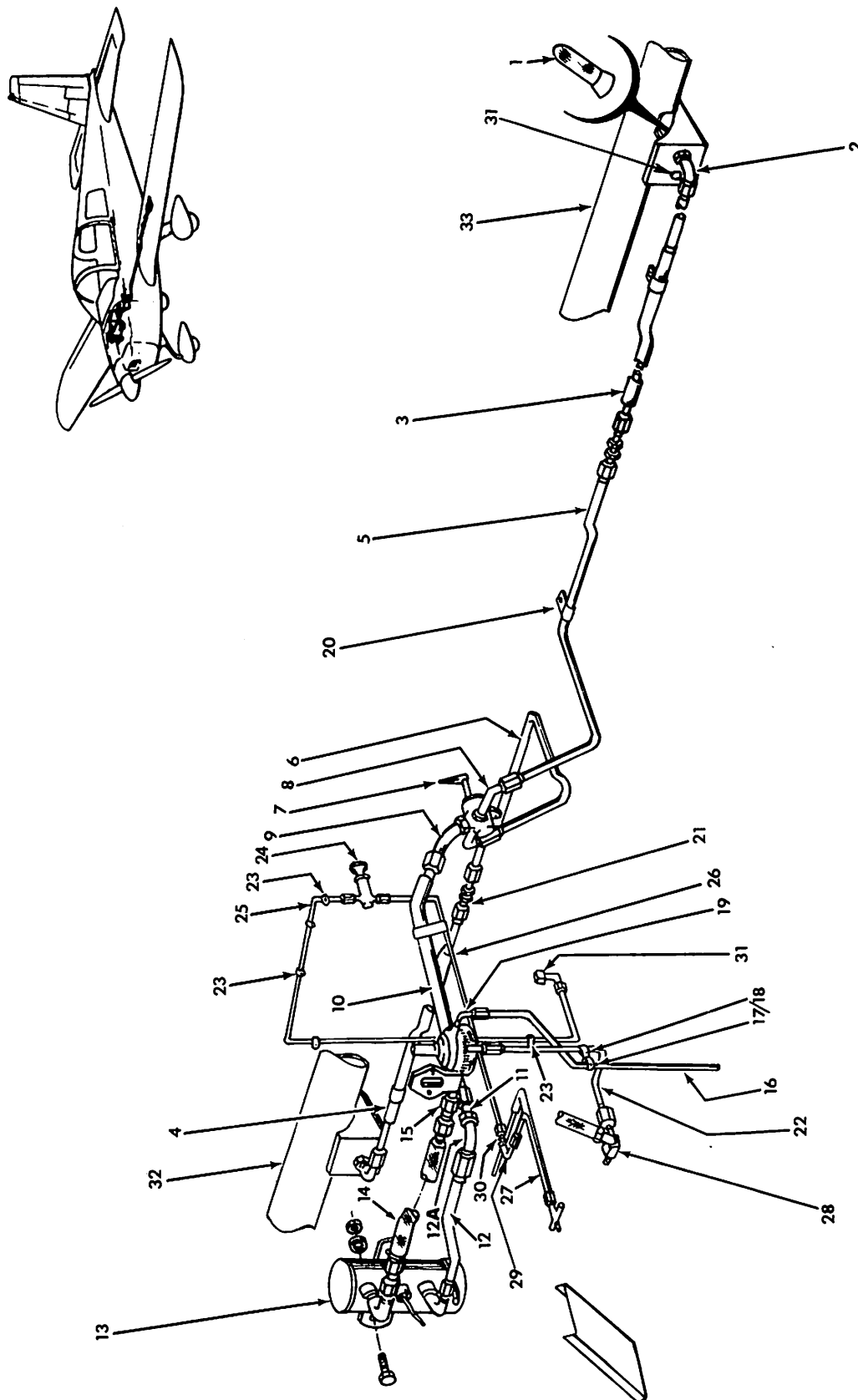
Fuel System Installation Figure 28-1
