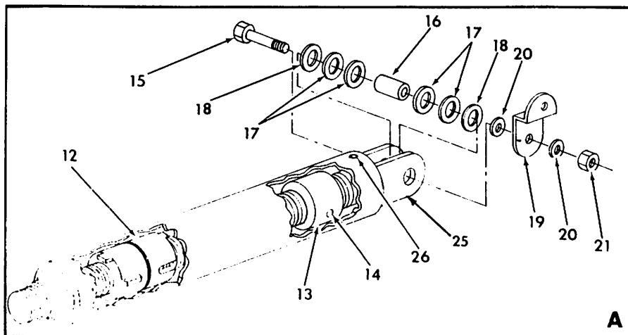
Flap Control Installation Figure 27-2
