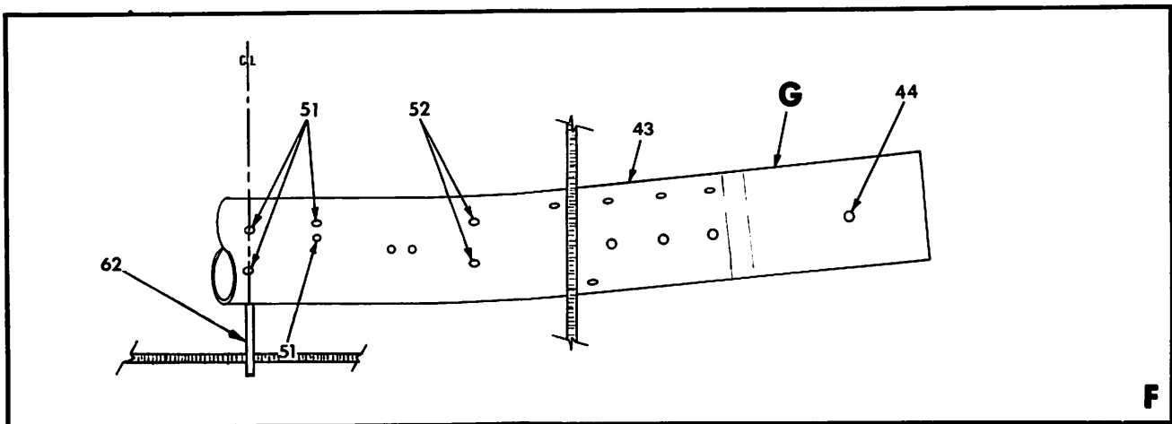
Fuselage Assembly (Sheet 2 of 4) Figure 53-1
