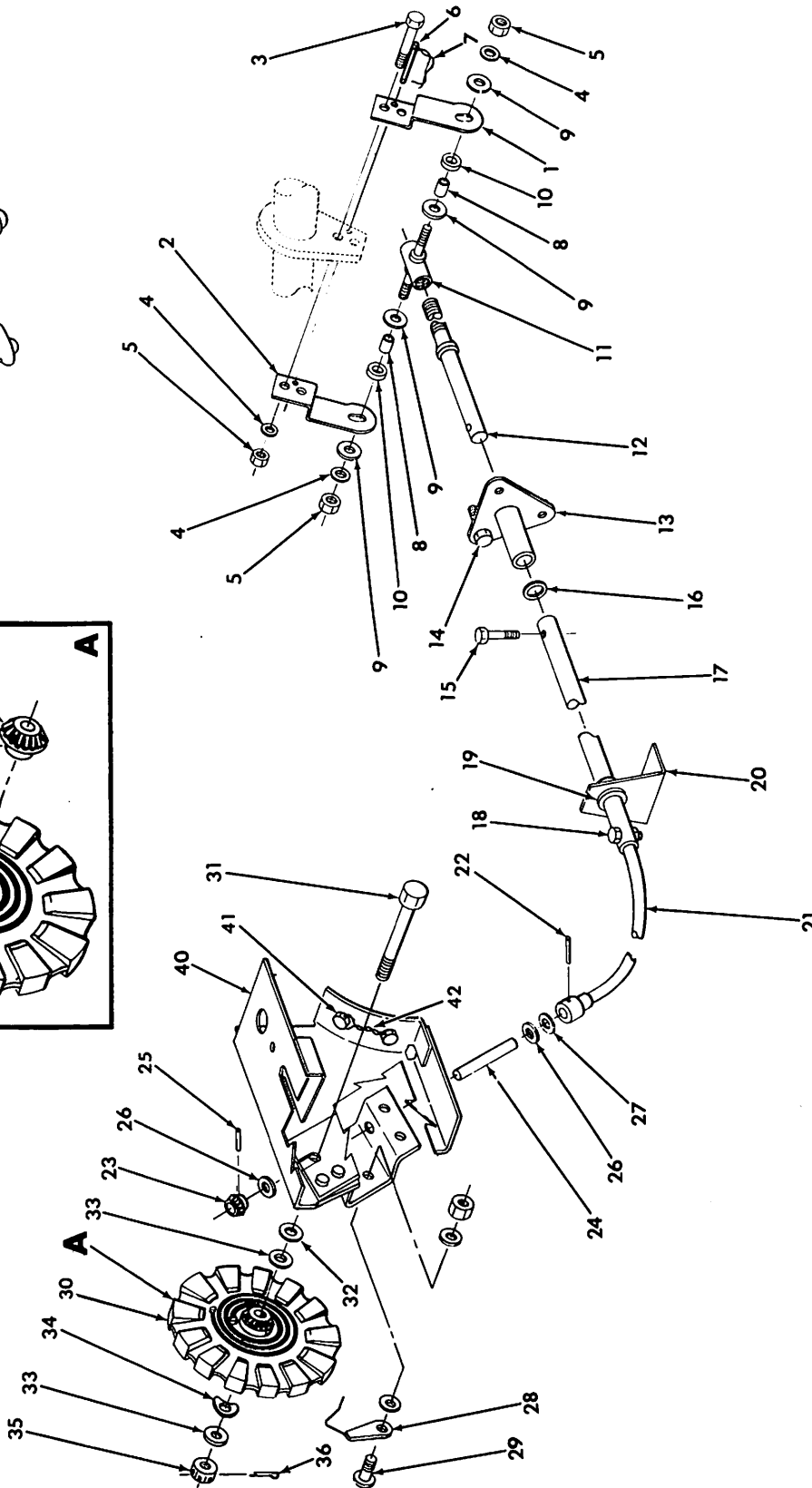
Trim Control Installation Figure 27-9
