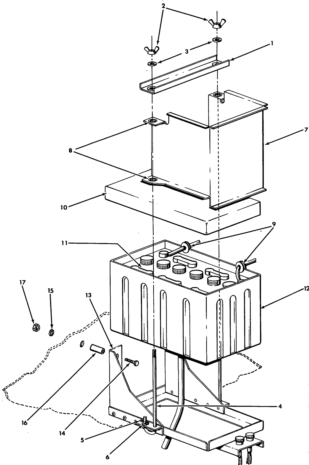
Battery Installation Figure 24-3
