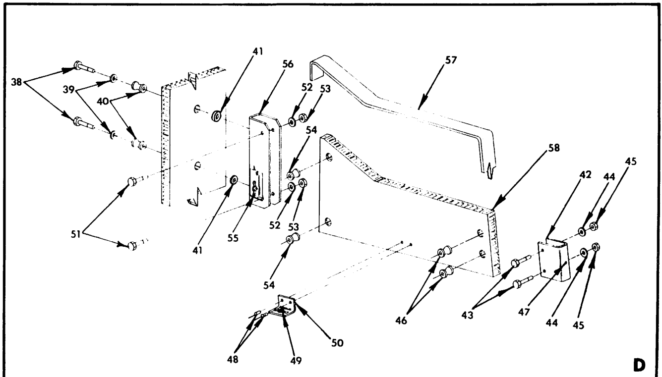
Wing Root Installation (Sheet 2 of 2) Figure 57-3
