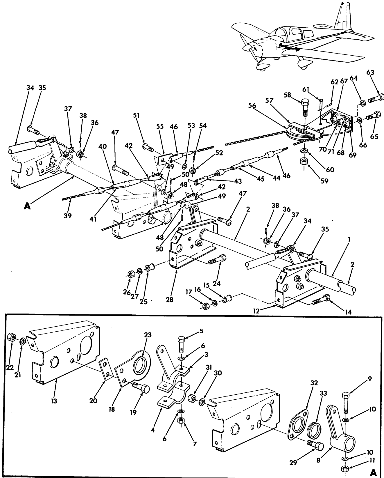
Flap Torque Tube Assembly Figure 27-5
