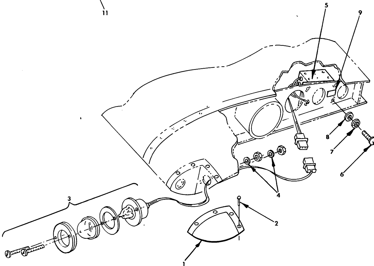
Strobe Light Installation Figure 33-3
