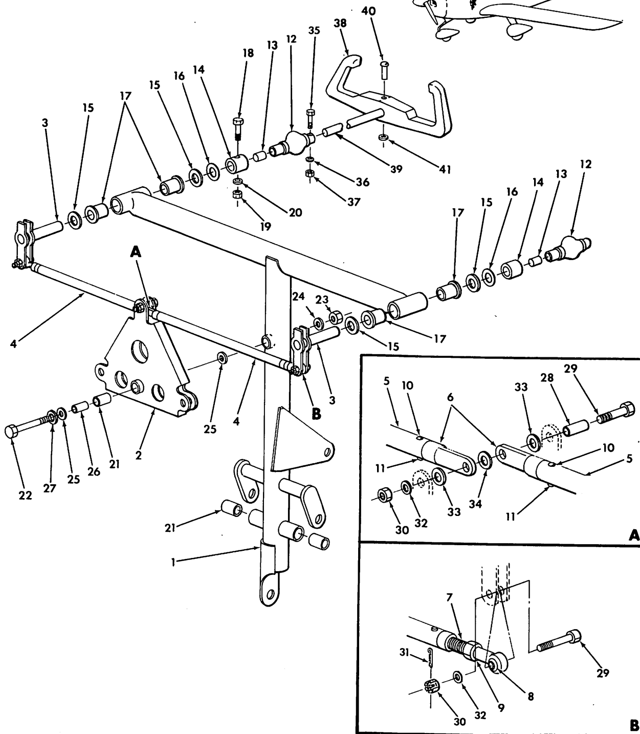
Control Column Assembly Figure 27-1
